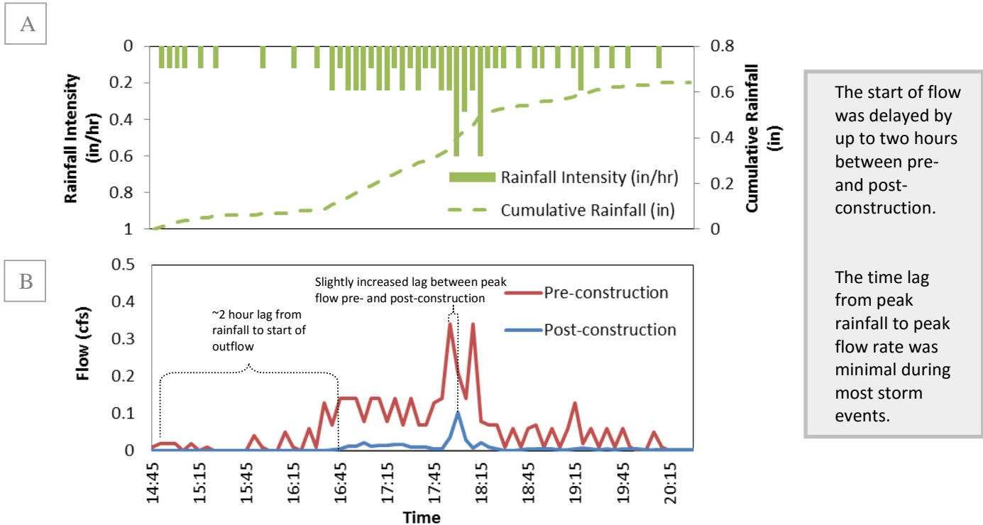
Figure 5. A) Rainfall intensity and cumulative rainfall at Newcomb South during a storm event on March 27-28, 2012. B) Storm hydrograph for Newcomb South with modeled pre-construction and monitored post-construction outflows during this storm event.
